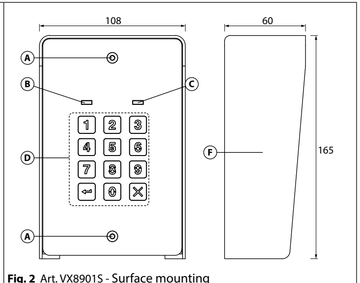
Fig. 2 Art. VX8901S - Surface mounting
