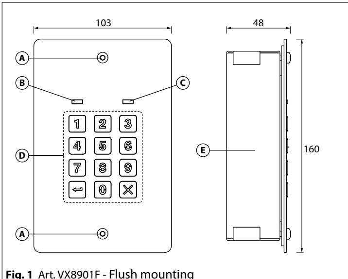
Fig. 1 Art. VX8901F - Flush mounting
